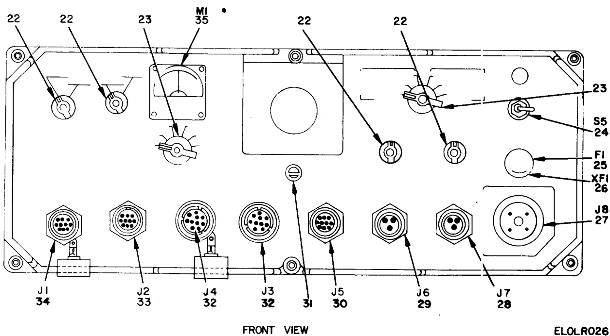
Figure 19. Panel Assembly, Front (Sheet 2 of 2).
