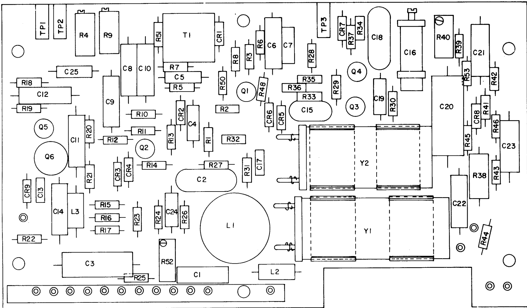
Figure 11. Transmitter Module, Printed Circuit Board (Transmitter Mixer Amplifier) A3A2 (Sheet 1 of 2).
