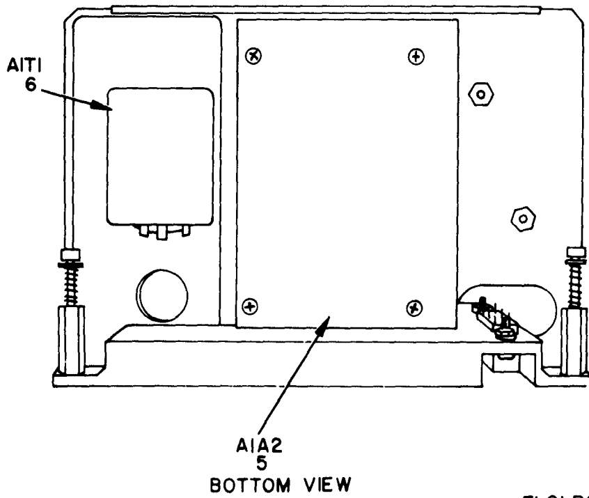
Figure 3. Receiver Audio, BFO, +20V Regulator Module.
