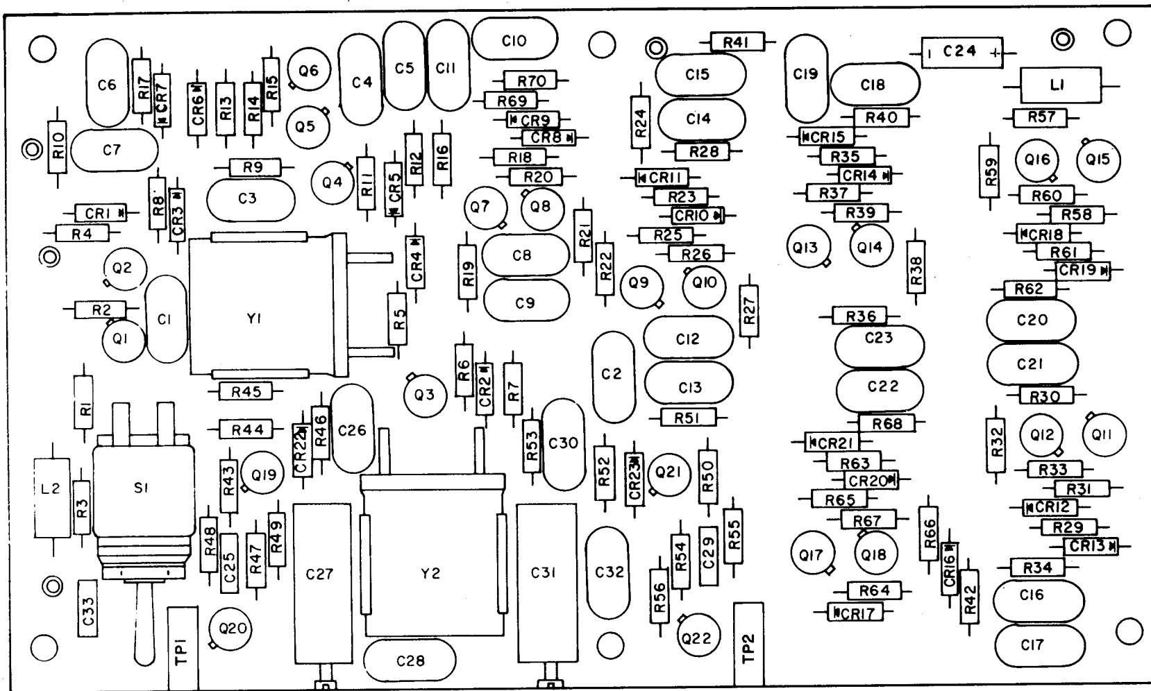
Figure 10. Transmitter Module, Printed Circuit Board (Transmitter Oscillator Divider) A3A1 (Sheet 1 of 2).
