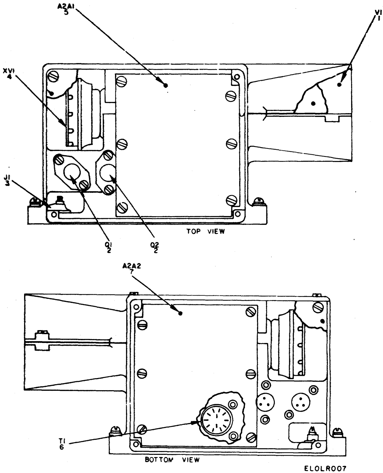
Figure 6. Scope Module A2.
