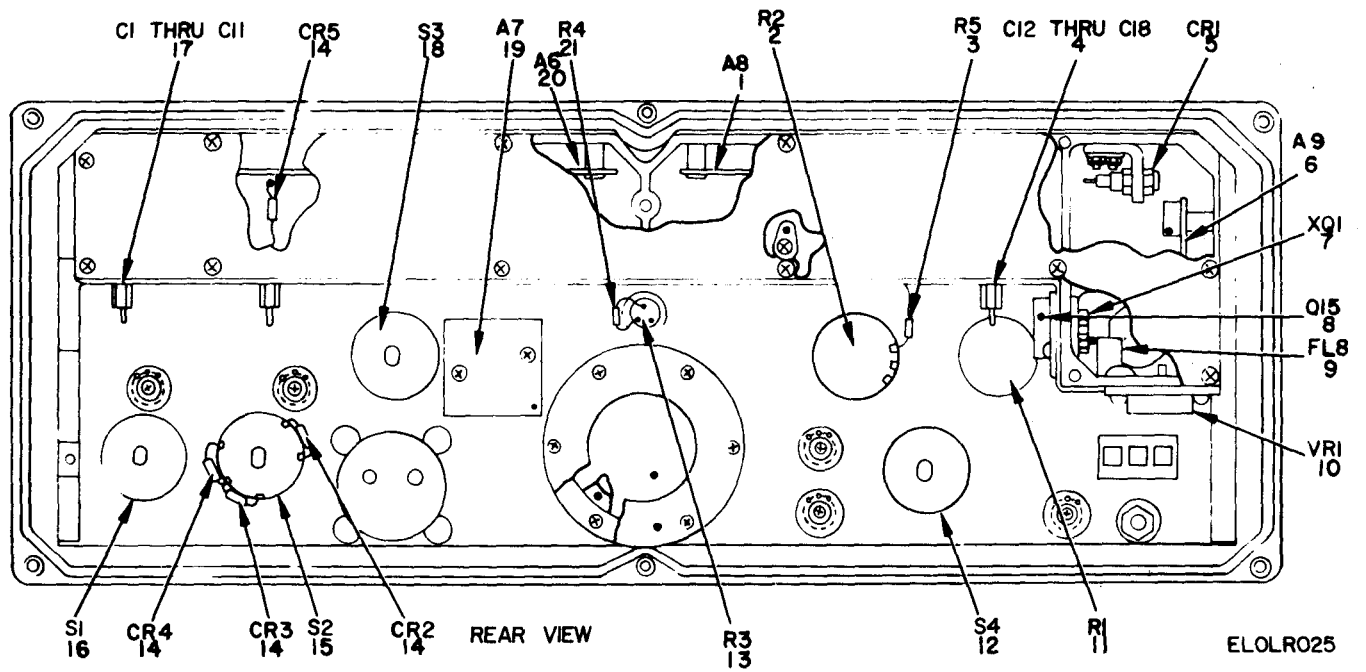
Figure 19. Panel Assembly, Front (Sheet 1 of 2).
