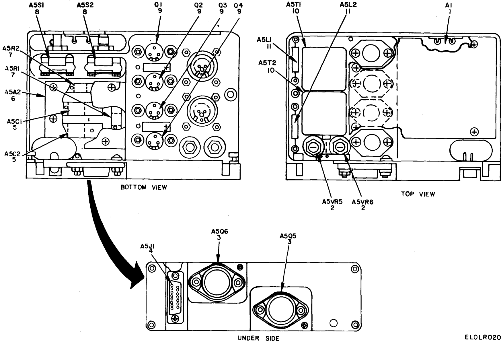
Figure 15. Loop Battery Module A5.
