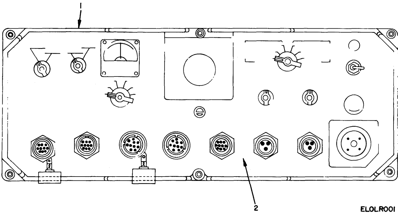
Figure 1. Modem, Radio Teletypewriter MD-522/GRC.
