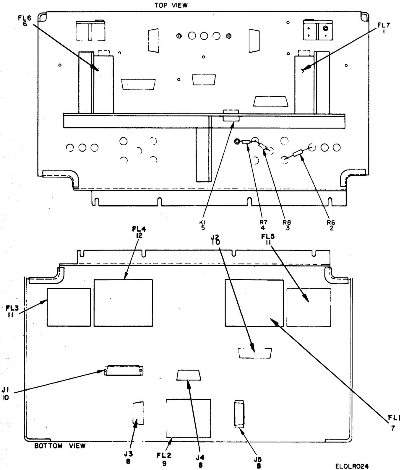
Figure 18. Chassis Assembly.
