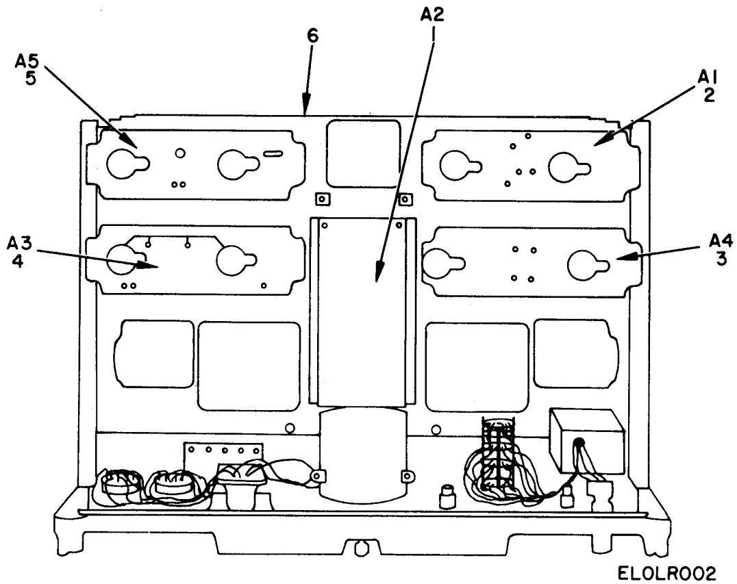
Figure 2. Modem, Radio Teletypewriter MD-522/GRC, Top View.
