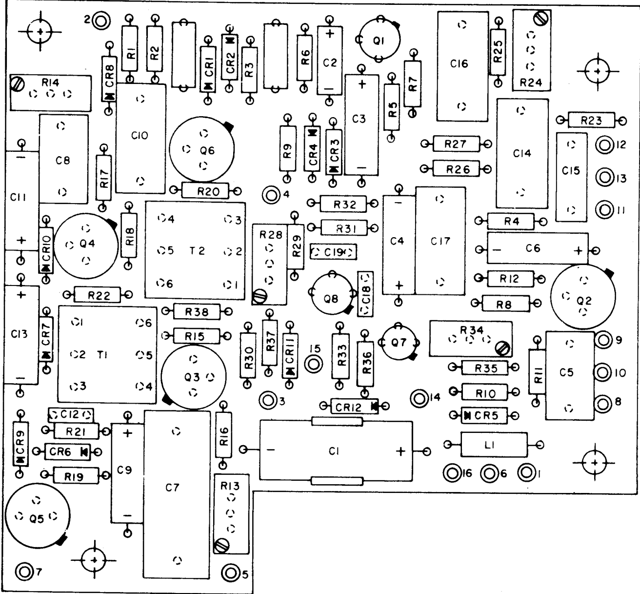
Figure 14. Receiver Module, Printed Circuit Board ( Diversity Receiver) A4A2 ( Sheet 1 of 2).
